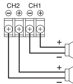
Speaker output terminals
