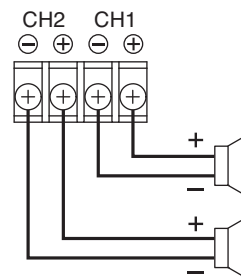
Speaker output terminals
