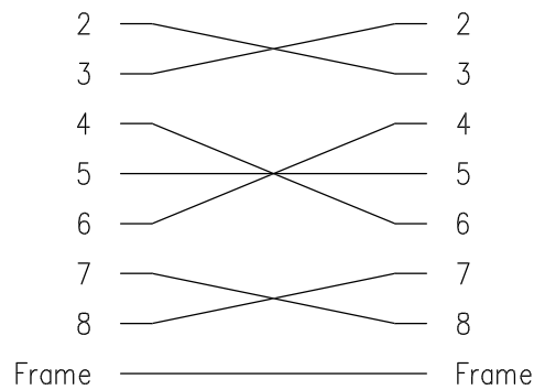
Wiring Diagram
